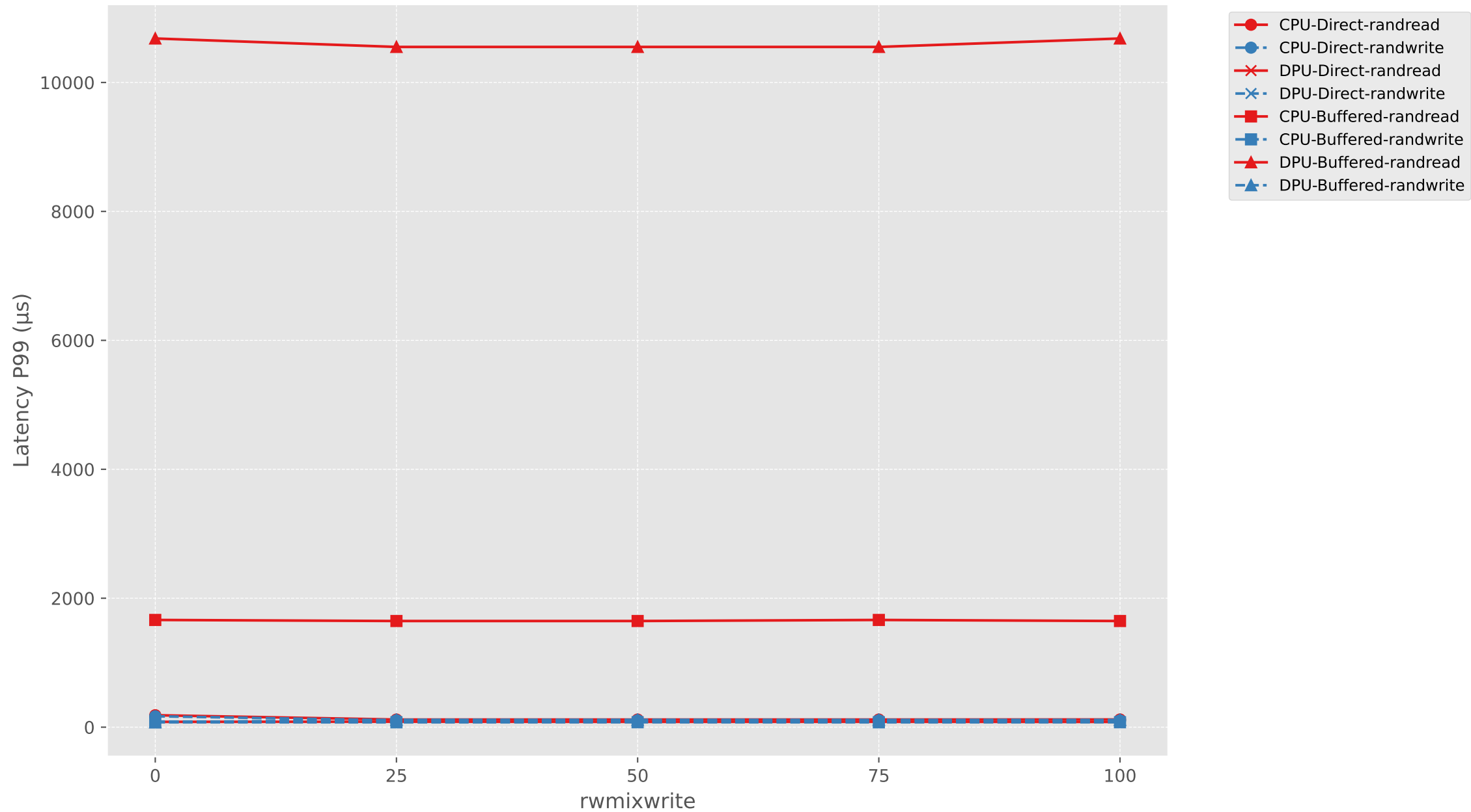
Latency P99 vs rwmixwrite (CPU vs DPU, Direct vs Buffered)
